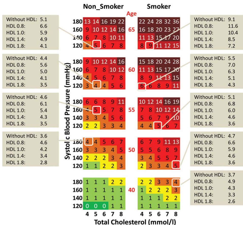
Fig. 5. Risk function without high-density lipoprotein-cholesterol (HDL-C) for men in populations at high cardiovascular disease risk, with examples of the corresponding estimated risk when different levels of HDL-C are included.
