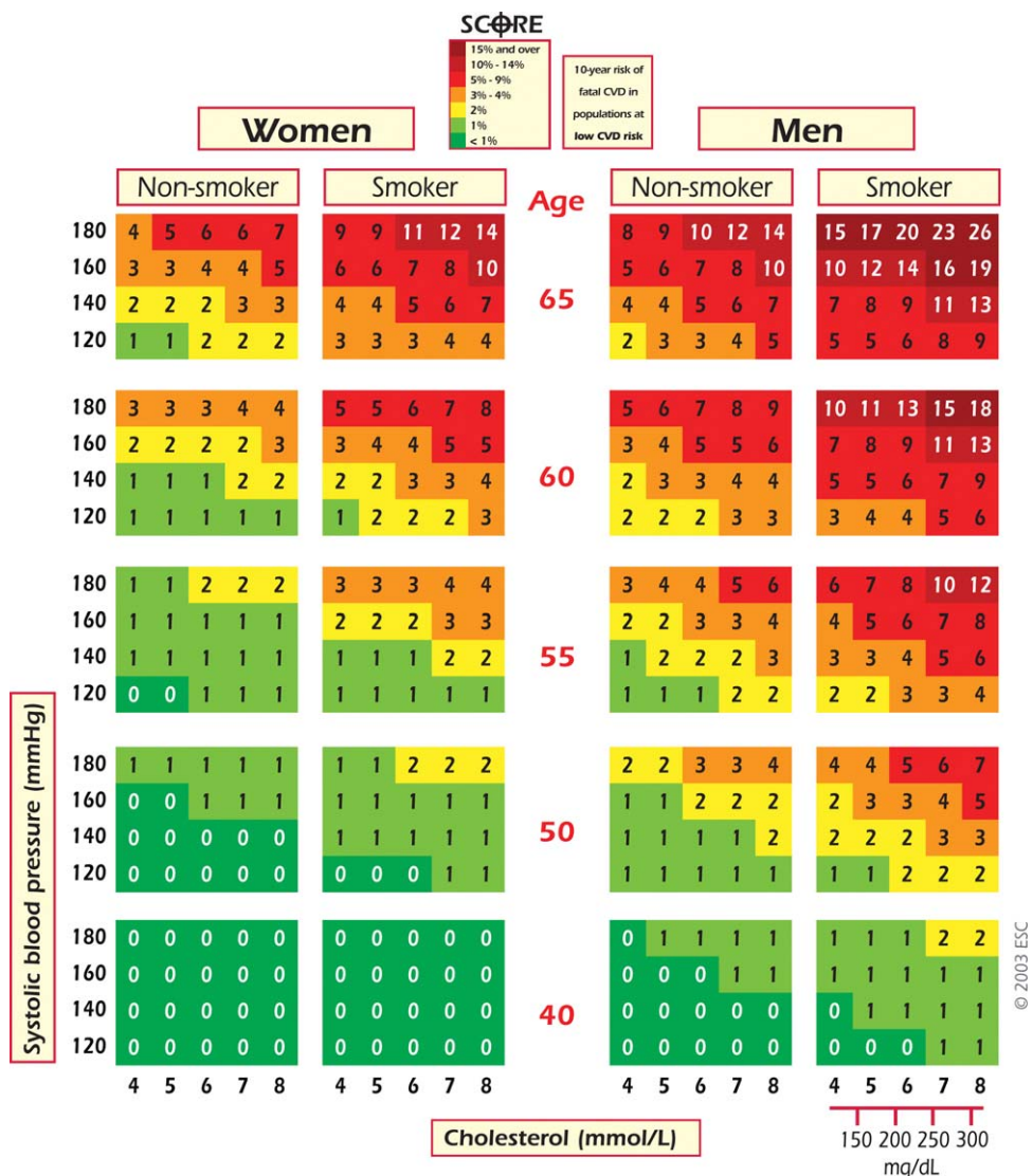
Fig. 2. SCORE chart: 10-year risk of fatal cardiovascular disease (CVD) in populations at low CVD risk based on the following risk factors: age, gender, smoking, systolic blood pressure, and total cholesterol. To convert the risk of fatal CVD to risk of total (fatal + non-fatal) hard CVD, multiply by 3 in men and 4 in women, and slightly less in old people. Note: The SCORE chart is for use in people without overt CVD, diabetes, chronic kidney disease, or very high levels of individual risk factors because such people are already at high risk and need intensive risk factor advice.
