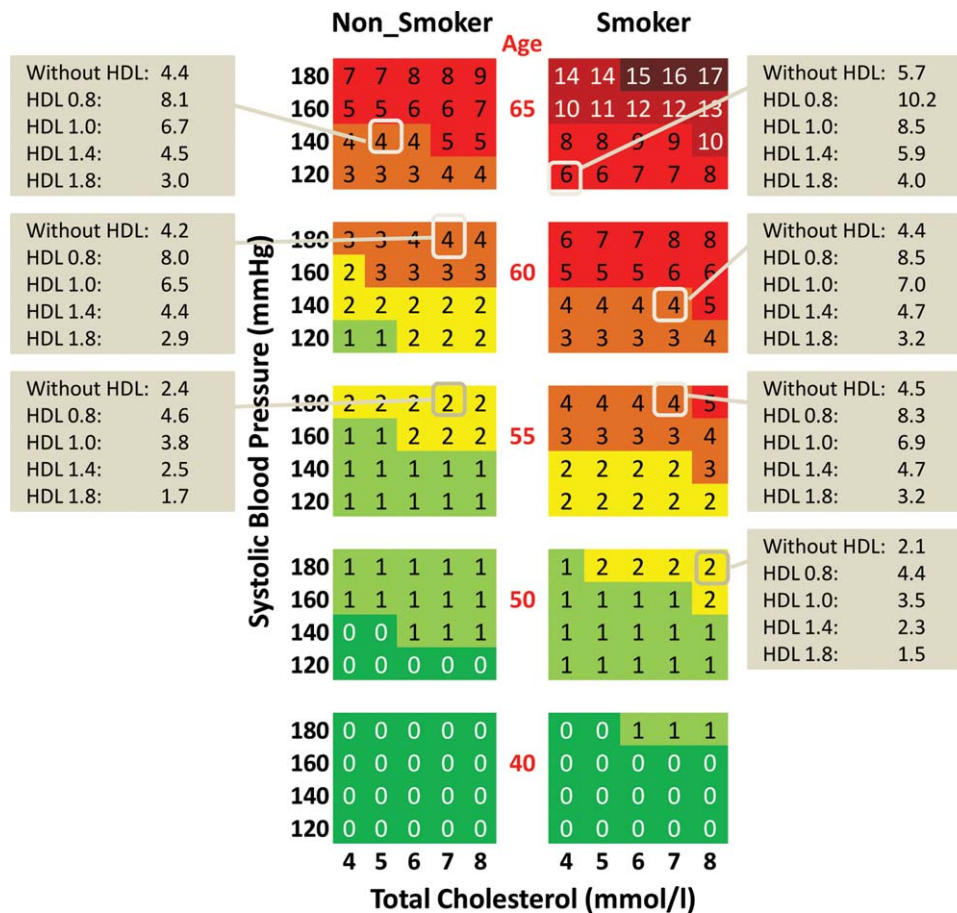
Fig. 4. Risk function without high-density lipoprotein-cholesterol (HDL-C) for women in populations at high cardiovascular disease risk, with examples of the corresponding estimated risk when different levels of HDL-C are included.
