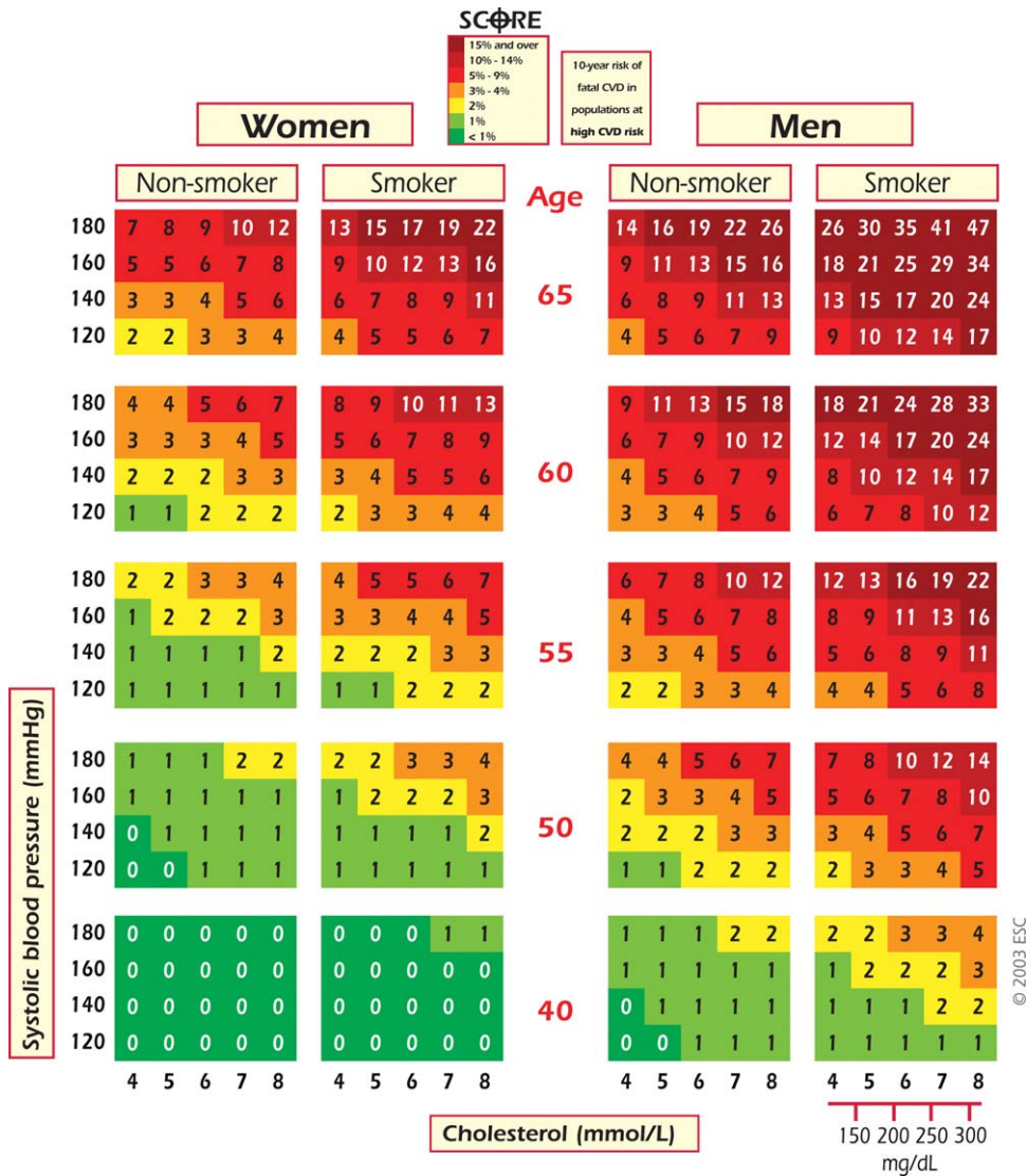
Fig. 1. SCORE chart: 10-year risk of fatal cardiovascular disease (CVD) in populations at high CVD risk based on the following risk factors: age, gender, smoking, systolic blood pressure, and total cholesterol. To convert the risk of fatal CVD to risk of total (fatal + non-fatal) hard CVD, multiply by 3 in men and 4 in women, and slightly less in old people. Note: The SCORE chart is for use in people without overt CVD, diabetes, chronic kidney disease, or very high levels of individual risk factors because such people are already at high risk and need intensive risk factor advice.
